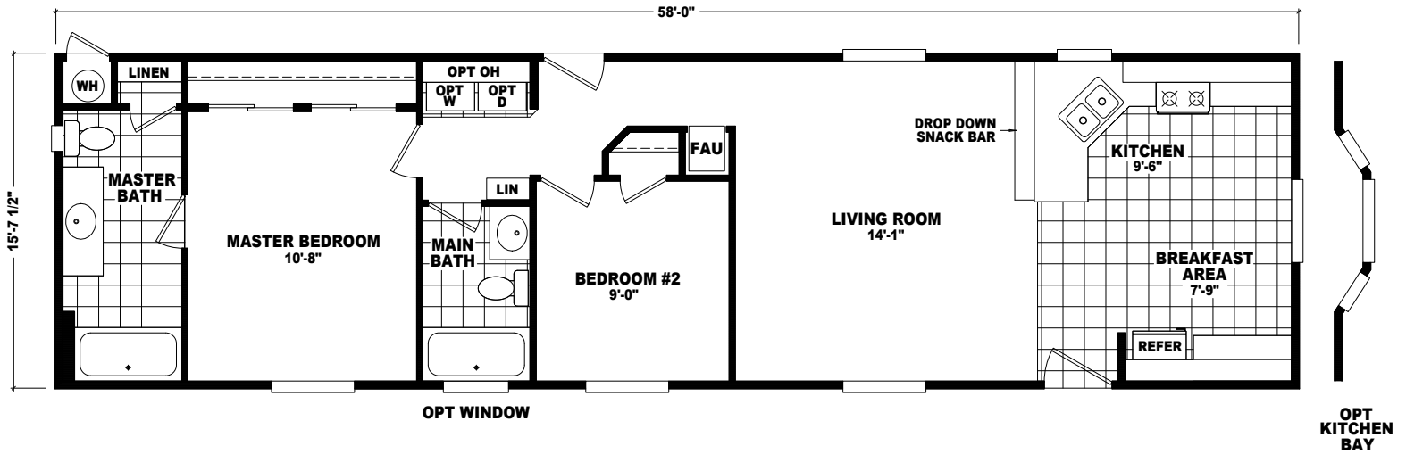
MODEL: DVS-5816A APPROXIMATELY 906 SQ. FT. 2 BEDROOM, 2 BATH
