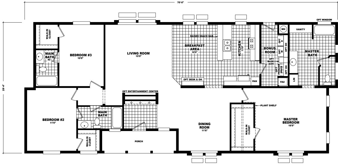
TR-1994A APPROXIMATELY 1994' SQ. FT. 3 BEDROOM, 3 BATH *Includes porch
