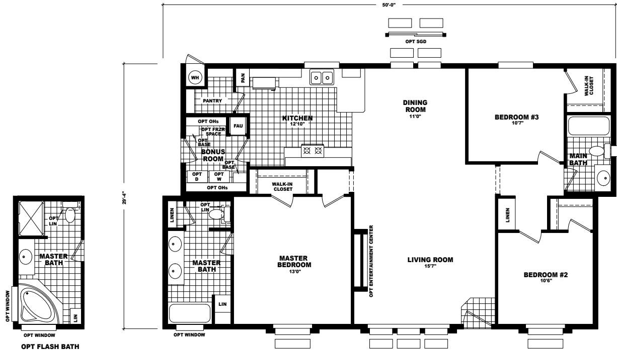
TR-1408A APPROXIMATELY 1408 SQ. FT. 3 BEDROOM, 2 BATH
