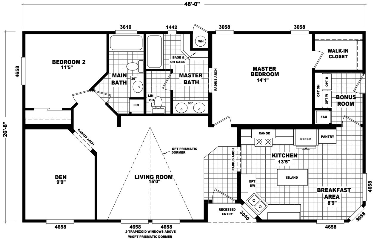
MODEL: SD-28483A APPROXIMATELY: 1262 SQ FT 3 BEDROOM, 2 BATH
