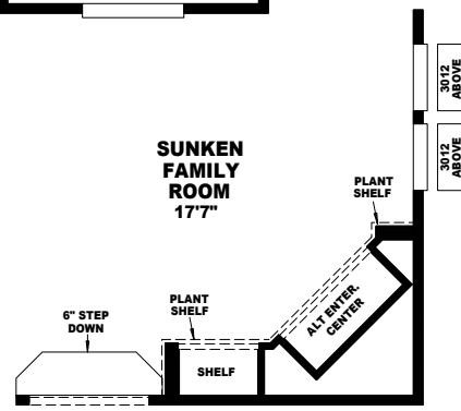
ALT ENTERTAINMENT CENTER @ SUNKEN FAMILY ROOM
