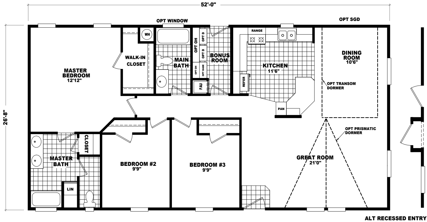
MODEL: 130BD28523B APPROXIMATELY 1386 SQ. FT. 3 BEDROOM, 2 BATH
