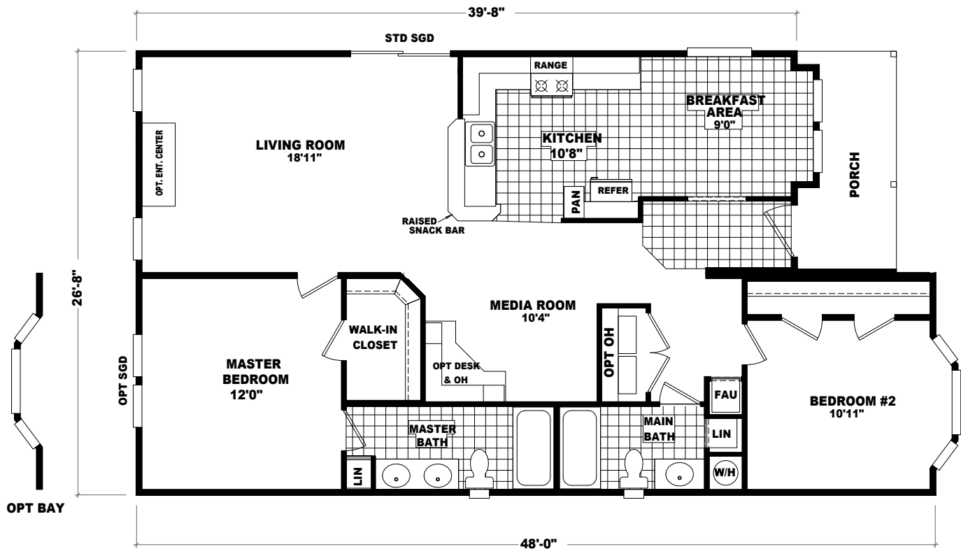
MODEL: 130BD28482L APPROXIMATELY 1148 SQ. FT. 2 BEDROOM, 2 BATH
