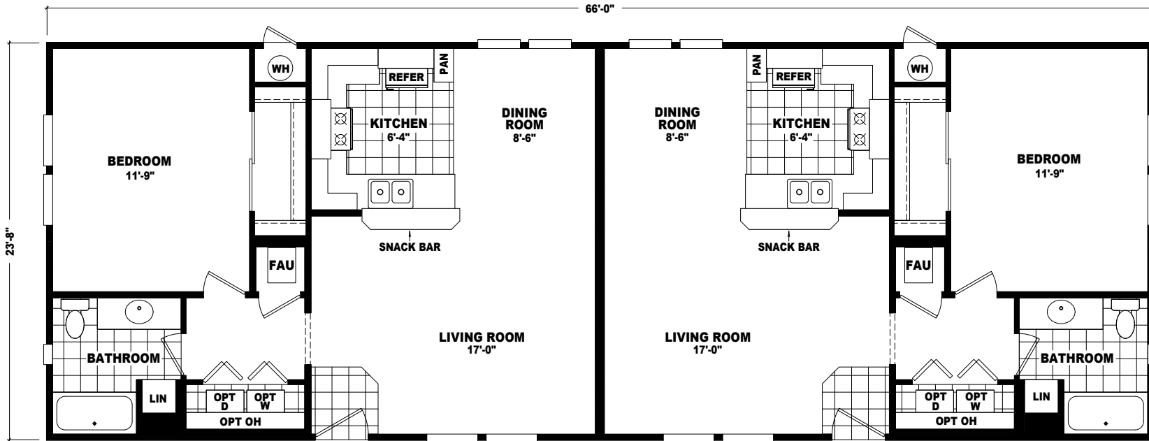
UNIT-B APPROXIMATELY 781 SQ. FT. 1 BEDROOM, 1 BATH
