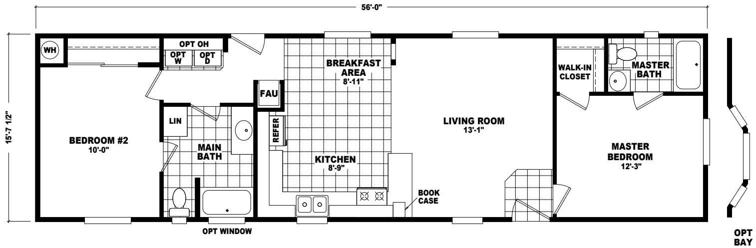
MODEL: DVS-5616A APPROXIMATELY 875 SQ. FT. 2 BEDROOM, 2 BATH
