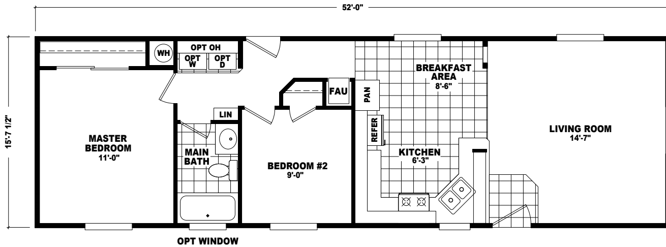
MODEL: DVS-5216B APPROXIMATELY 812 SQ. FT. 2 BEDROOM, 1 BATH
