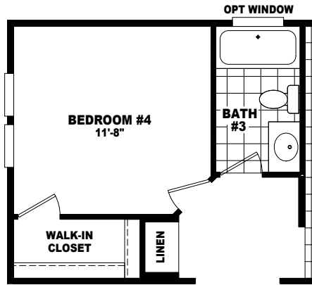
OPT 4th BEDROOM & 3rd BATHROOM
