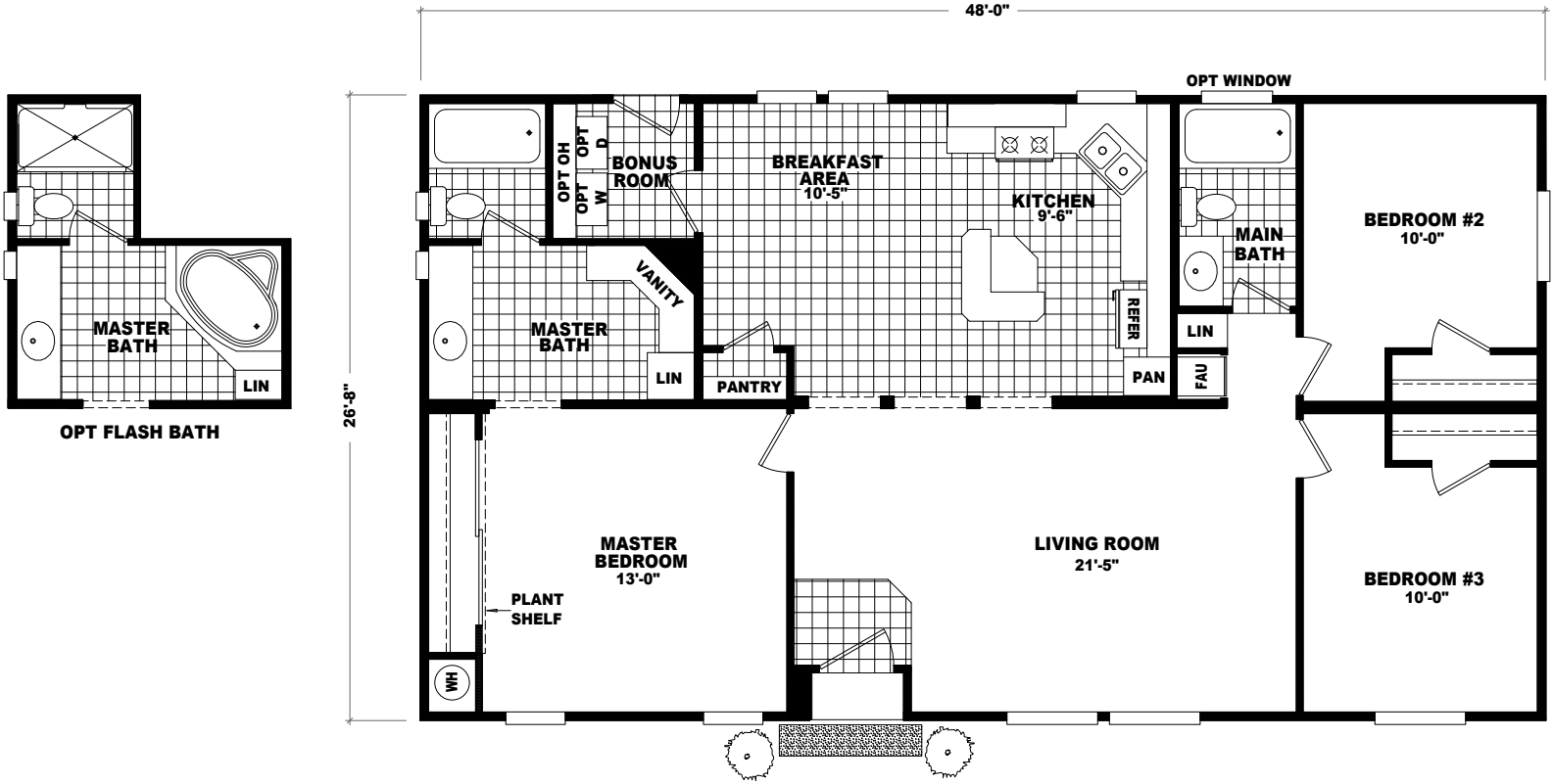
MODEL: CPS-4828A APPROXIMATELY 1280 SQ. FT. 3 BEDROOM, 2 BATH
