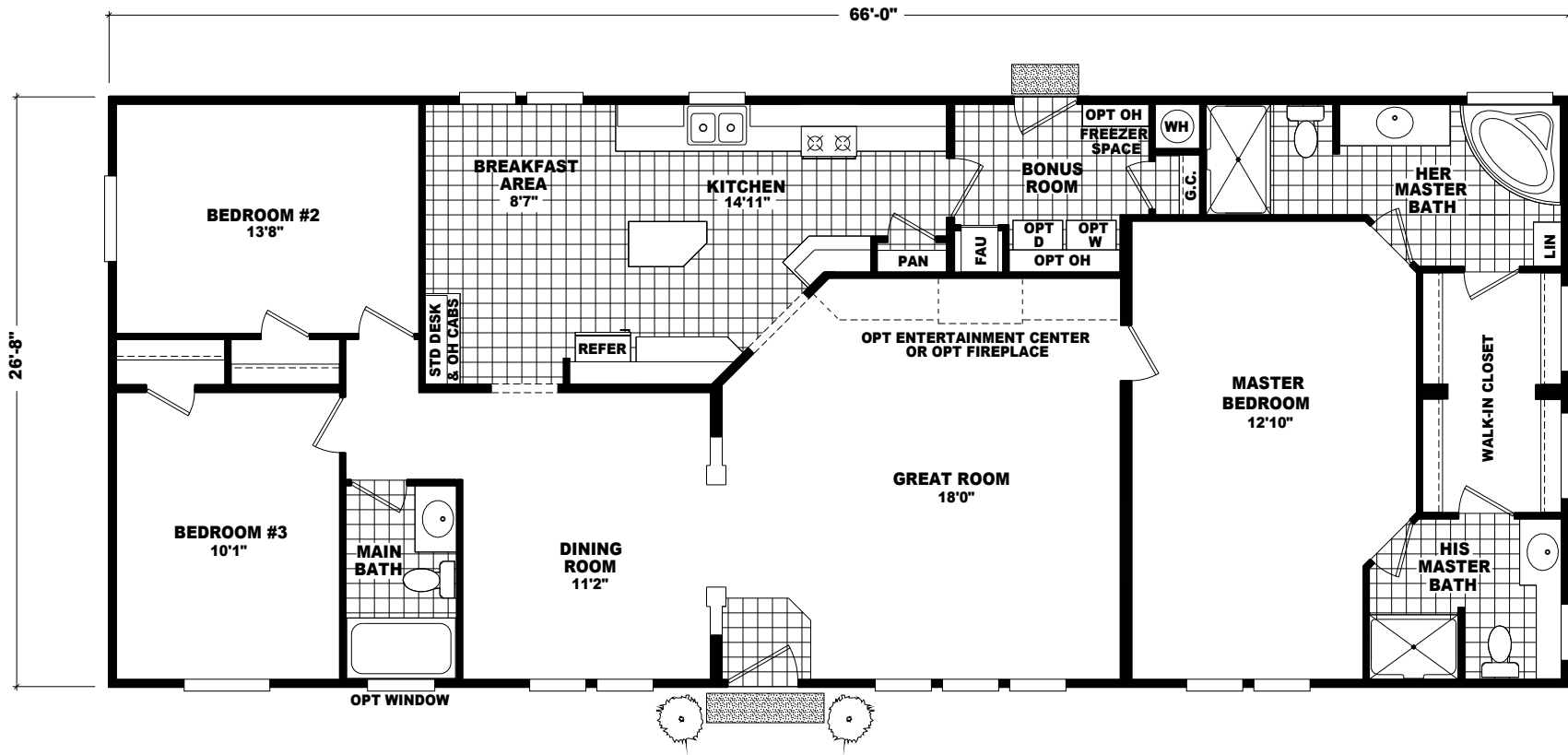
MODEL: CLE-6628A APPROXIMATELY 1760 SQ. FT. 3 BEDROOM, 3 BATH
